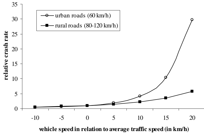
Relative accident rate on urban roads [37][36] and rural roads [38] for vehicles going faster and slower than average speed (=0) [36].
